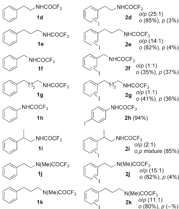
Scheme 1. Regioselectivity in the iodination of N -trifluoroacetylammides. The o/p ratios were determined by GC and/or ^1\text{H} NMR spectroscopic analysis of the crude reaction mixtures; the yields of the individual isomers after isolation by chromatographic separation are given.
