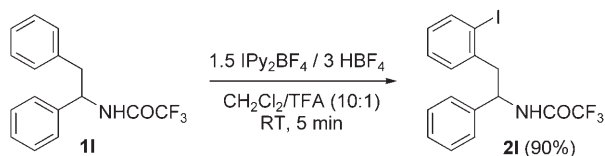
Scheme 2. Chemo- and regioselective iodination of 1l .
