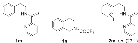
Scheme 3. Model compounds.
